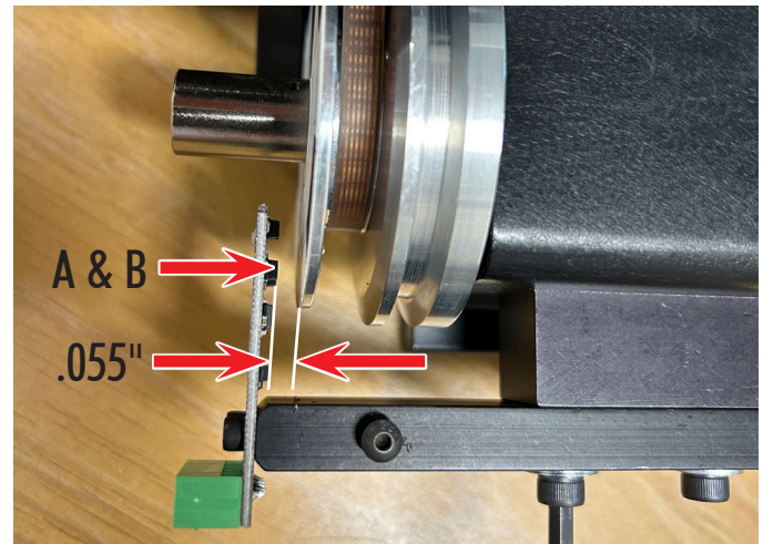
FIGURE 1—Showing .055” gap between the tach sticker and the A & B LEDs.
