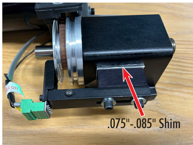
FIGURE 3—Showing the .075"-.085" shim stock installed between the headstock and the encoder headstock spacer.
