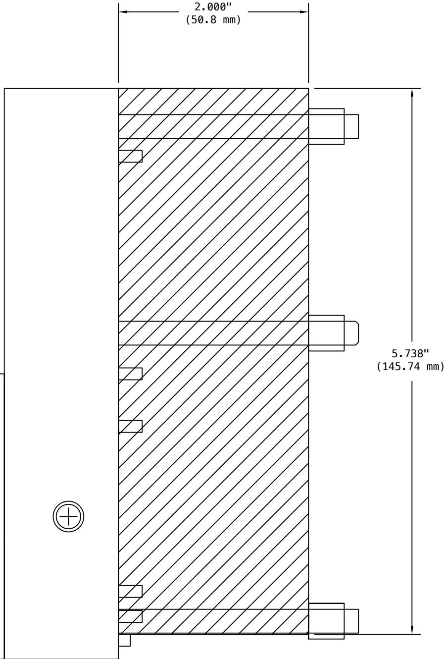
SIDE VIEW
