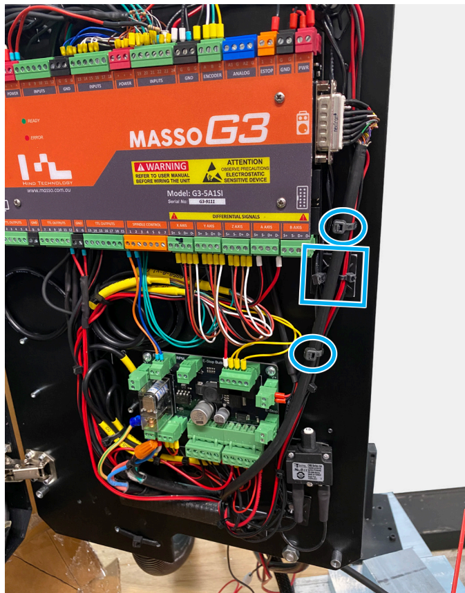
FIGURE 3—The blue square shows the location of the square zip tie mount on the control housing. The blue ovals show additional zip tie locations.
