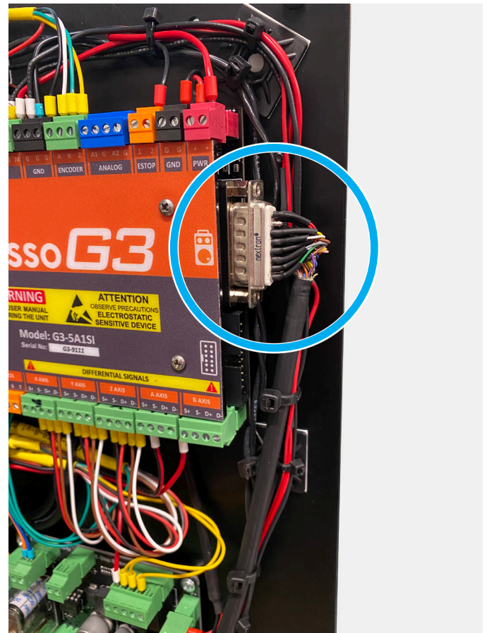
FIGURE 2—The blue circle shows the MPG DB15 male connector hooked up to the DB15 female connector.
