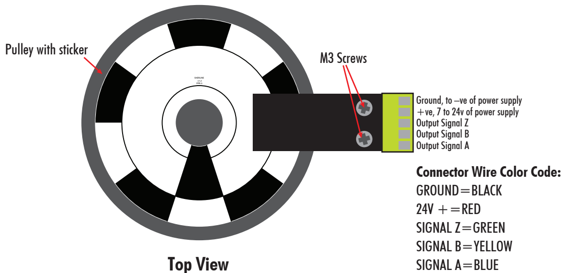
FIGURE 2—The Top View shows the wire connections and the wiring color code.
