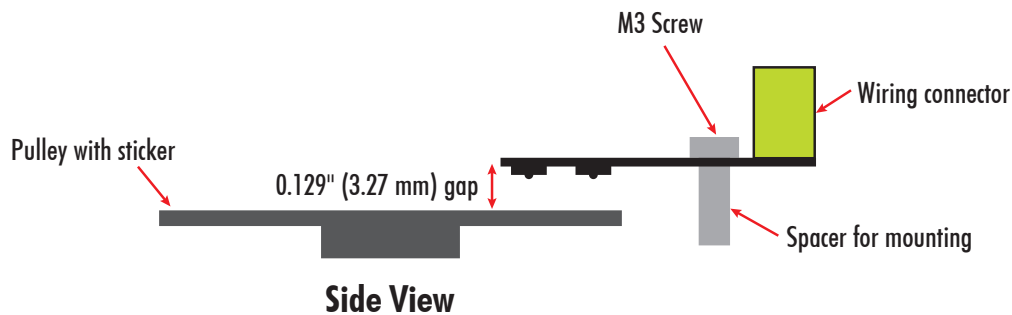
FIGURE 1—The Side View of the Optical Encoder shows the gap setting. M3 screws are equivalent to a 4-40 tap size.
