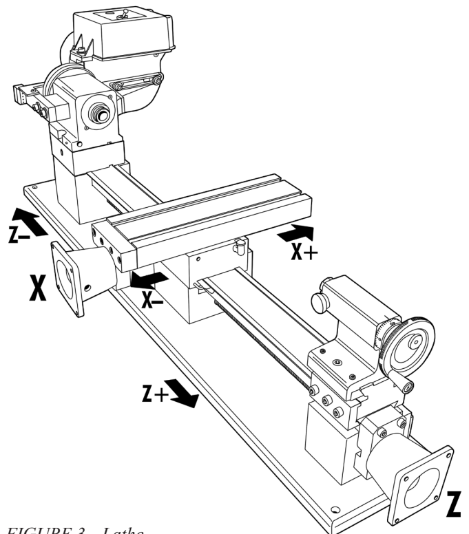
FIGURE 3—Lathe
