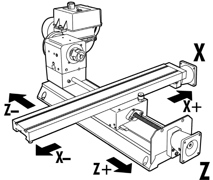
FIGURE 2—Chucker Lathe
