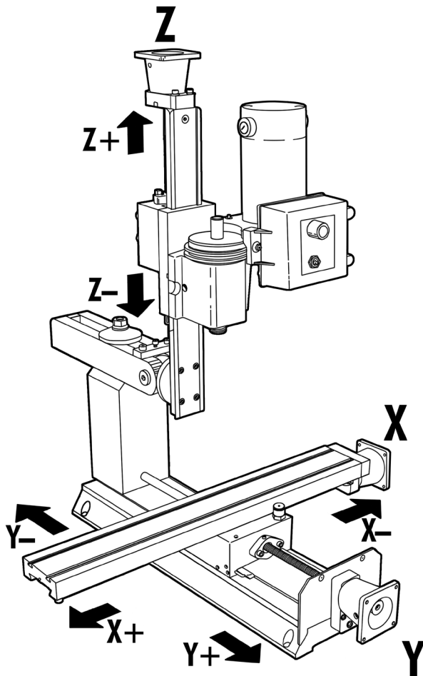
FIGURE 1—Mill
